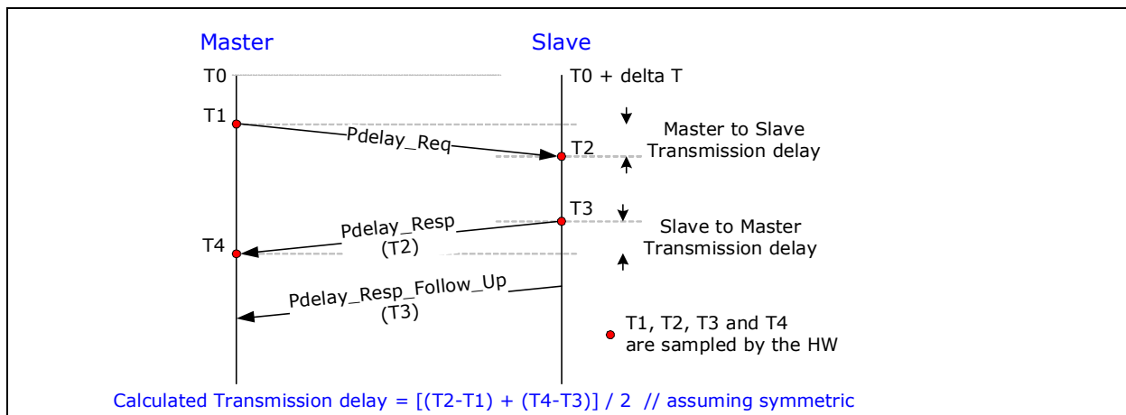
Figure 8-12. PDelay Flow
